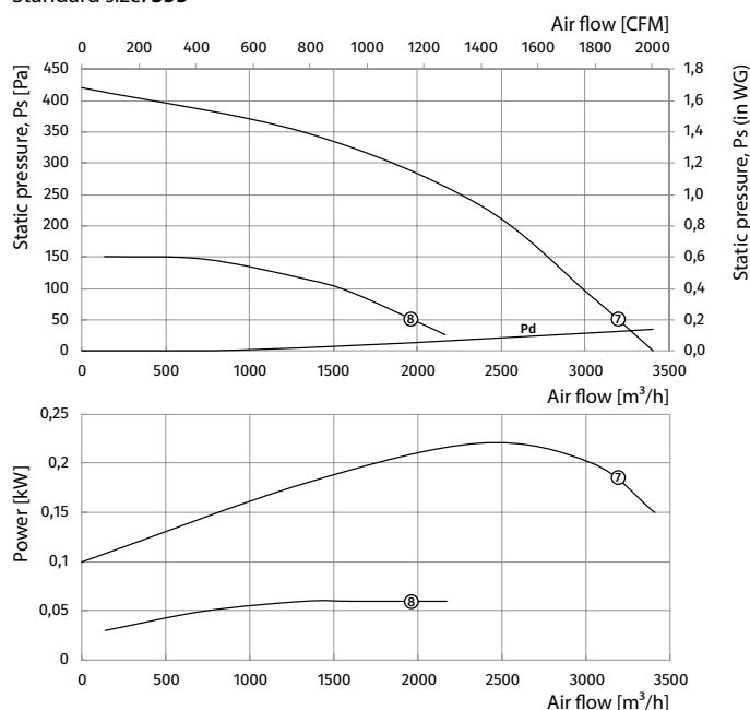
Standard size: 355
