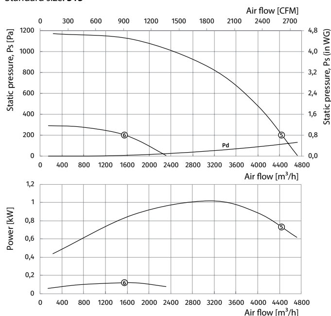
Standard size: 315
