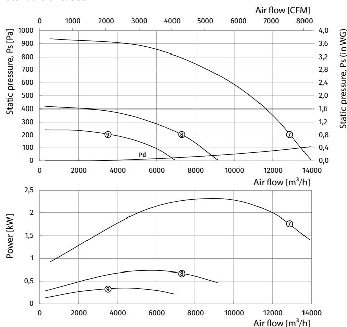
Standard size: 560
