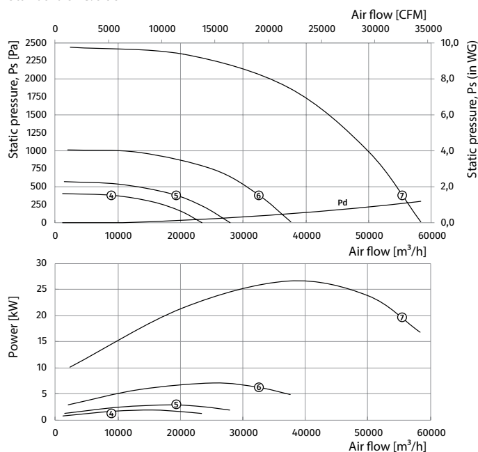
Standard size: 1120
