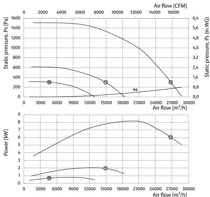
Standard size: 710
