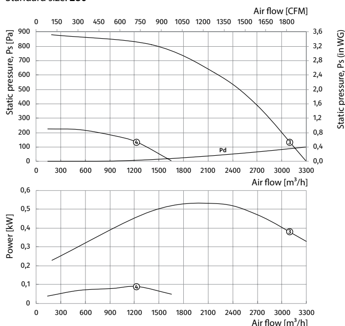
Standard size: 280
