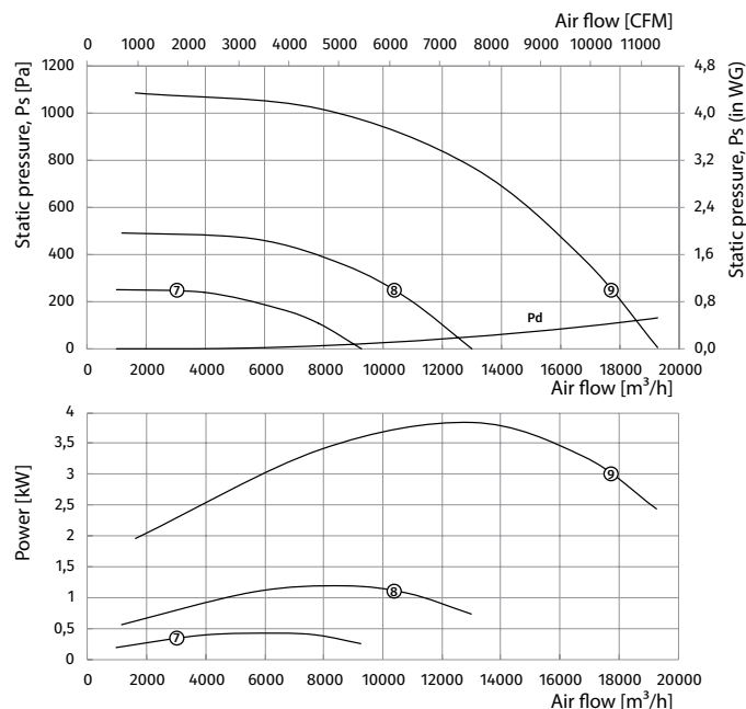
Standard size: 630
